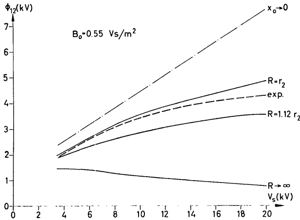
Fig. 2 Voltage \Phi_{12} across the rotating plasma in the Ixion as a function of the second capacitor bank voltage V_s . The value of B_0 is 0.55 Vs/m 2 . Dashed curves give experimental results for the peak values of \Phi_{12} according to BAKER and HAMMEL [9]. Full curves give calculated voltage characteristics at full charge transfer for an assumed plasma density \rho_0 = 5 \times 10^{-5} kg/m 3 and an effective axial length L = 0.2 m. An infinitely conducting chamber wall corresponds to R = r_2 and a non-conducting wall to R \rightarrow \infty . The radial diffusion of the magnetic flux across the wall at r = r_2 can be simulated by a proper choice of R . The intermediate full curves demonstrate the case R = 1.12 r_2 . Dot-and-dash lines give the characteristics which would have been obtained for a field of infinite rigidity.
