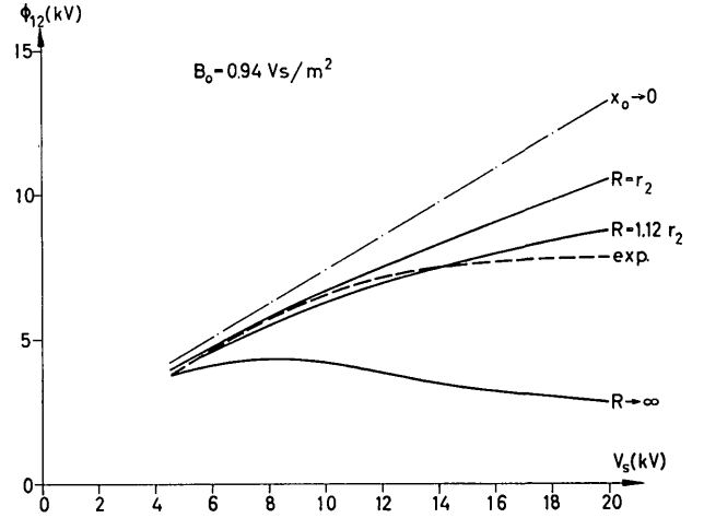
Fig. 3 Voltage \Phi_{12} across the rotating plasma in the Ixion as a function of the second capacitor bank voltage V_s . Same as Fig. 2, but with B_0 = 0.94 Vs/m 2 .
